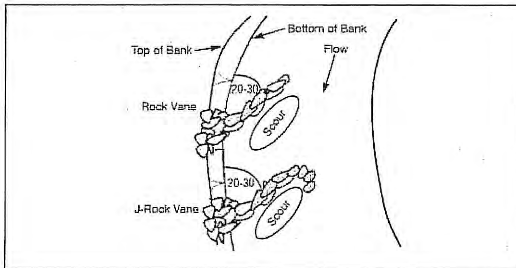
Figure 4-15. Rock and J-Rock Vane
