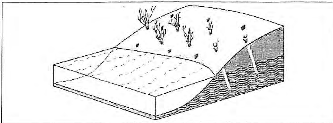
Figure 4-10. Live Stakes
