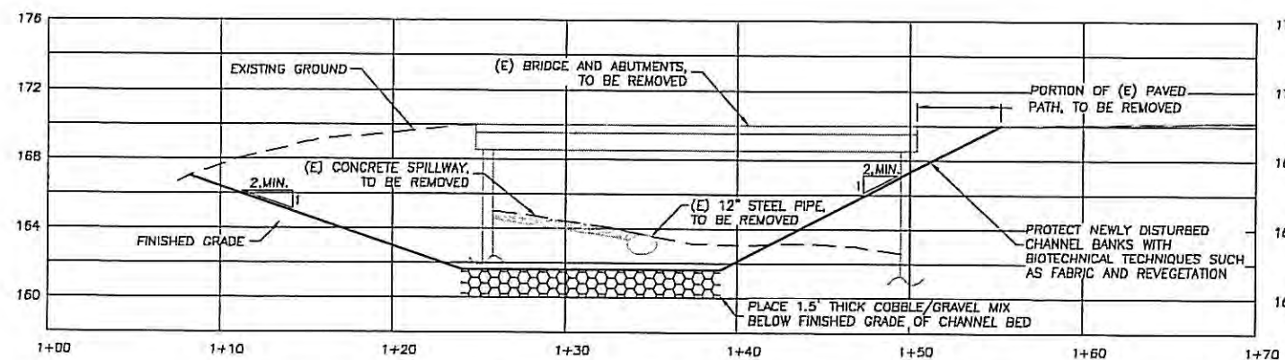
BRIDGE SECTION
