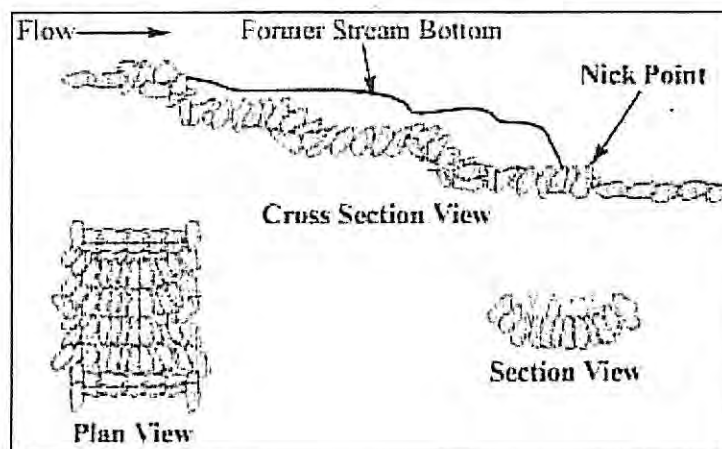
Figure 4-23. Step Pools
