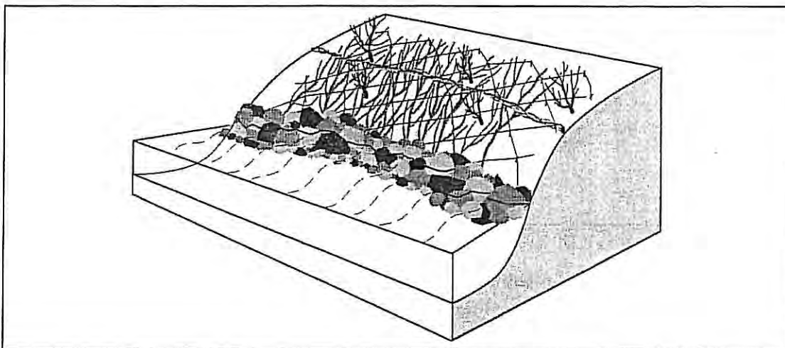
Figure 4-6. Brush Mattresses
