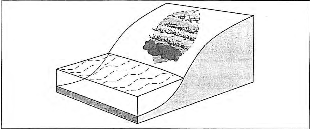
Figure 4-3. Brush Packing
