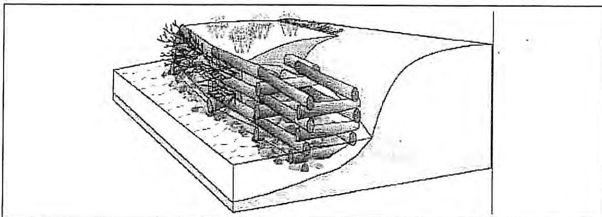
Figure 4-8. Live Cribwalls
