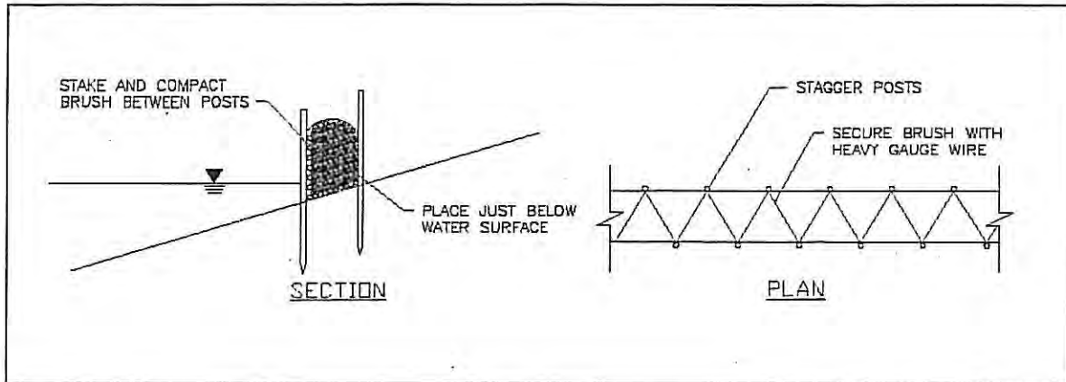
Figure 4-5. Brush Boxes
