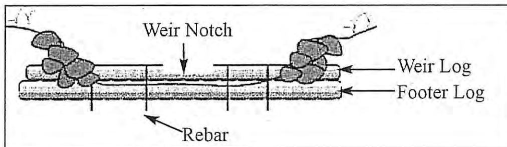
Figure 4-26. Log Drop
